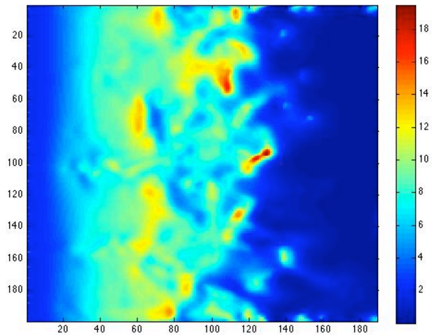
WRF-generated accumulated rainfall (mm)
