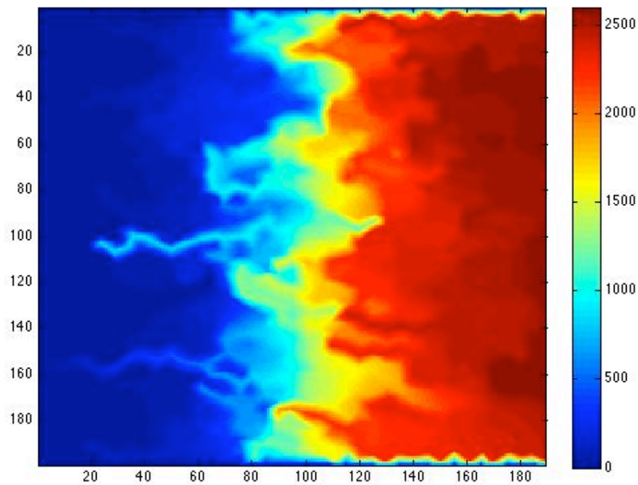
CHILD-generated topography (m)
