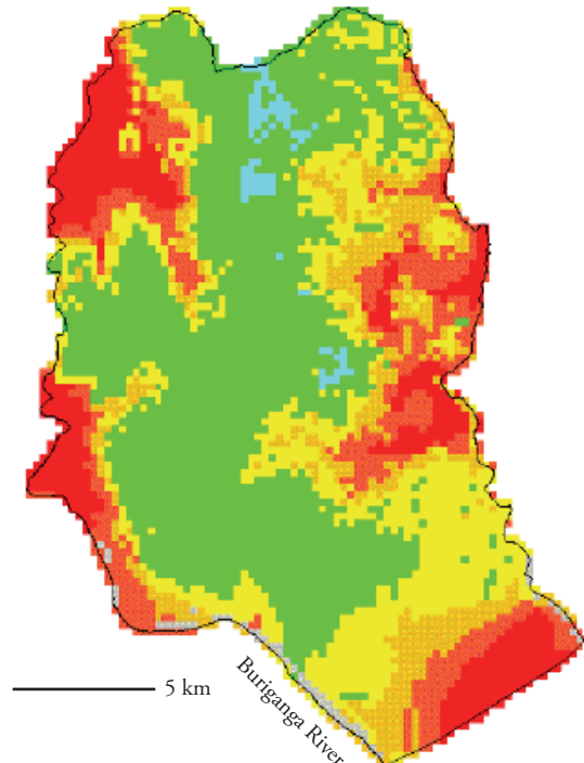
b) Soil class (CDMP, 2009)
