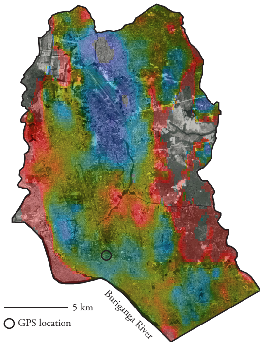
a) InSAR compaction measurements
