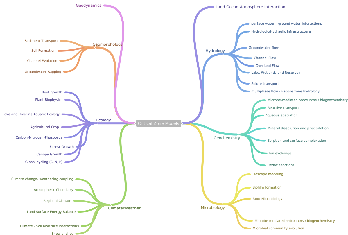
Figure 9 Mindmap of CSDMS-CZO related models
