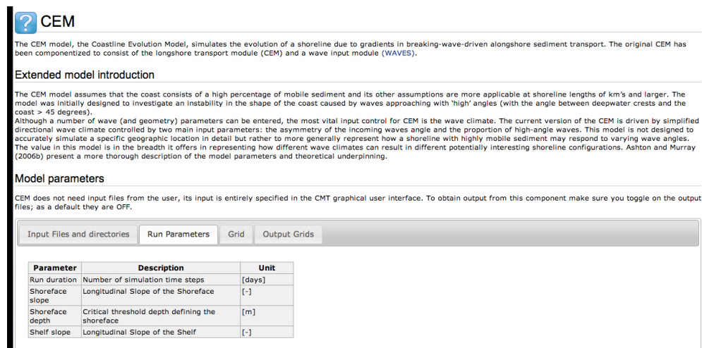
Figure 4. Detailed model description of the CEM-Coastline Evolution Model as displayed within WMT.
