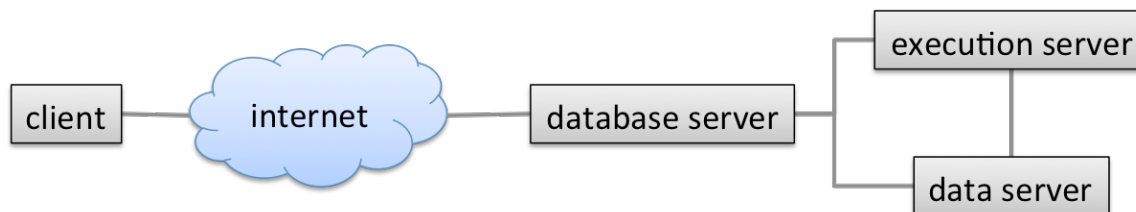
Figure 3 The relationship between the WMT client and the WMT server.
