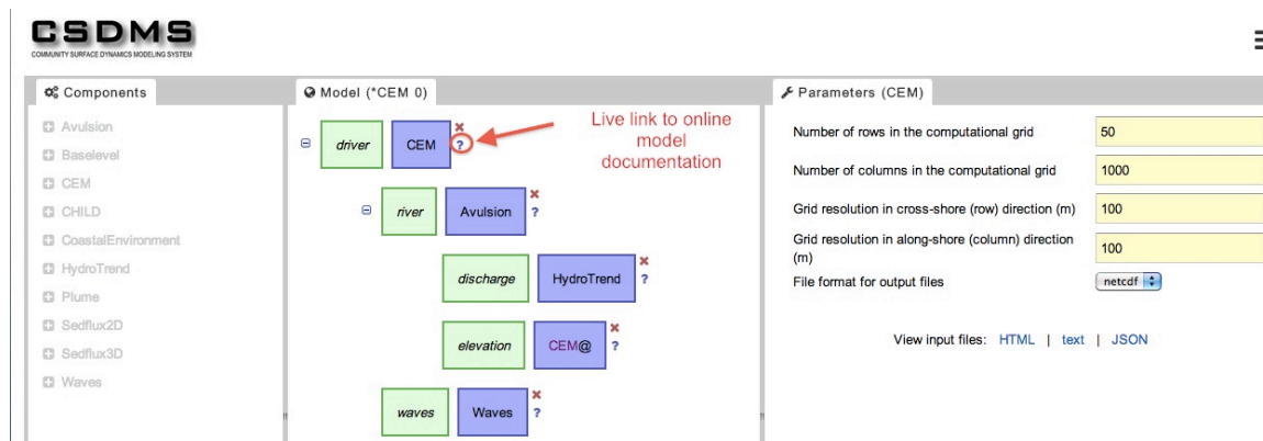
Figure 6 All components in the WMT have easy live links to online detailed documentation maintained on the CSDMS wiki
