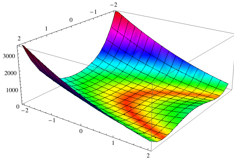
Figure 1. The Rosenbrock function, a classic test problem in optimization.
