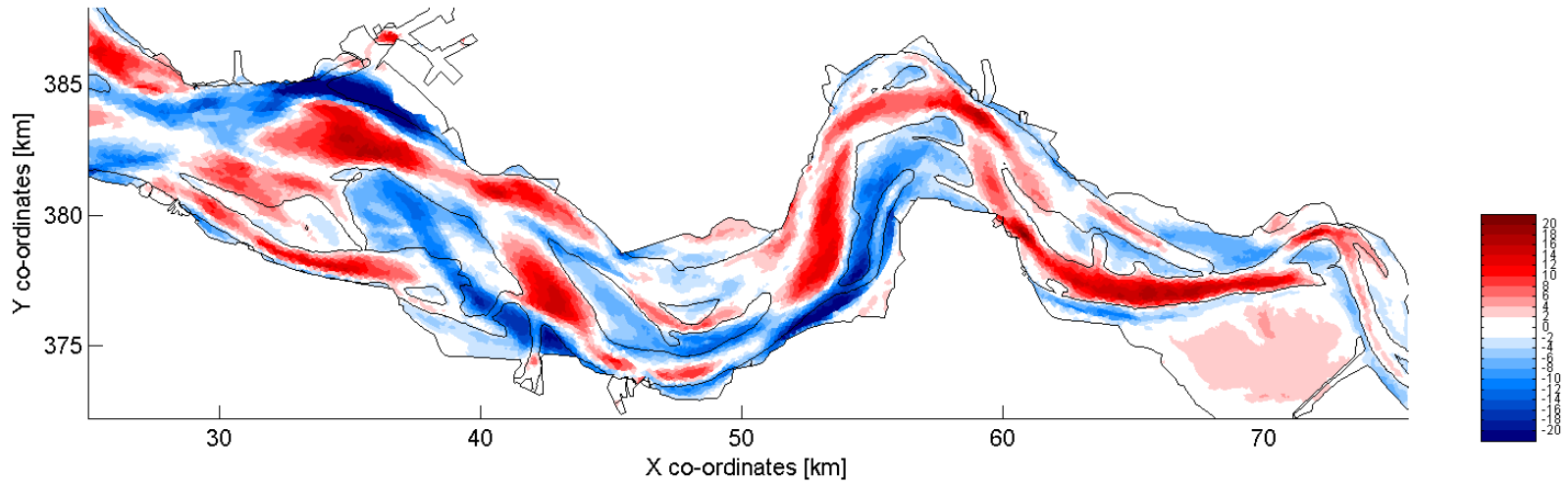
Model Run 2; erosion/sedimentation 1860 - 1970
